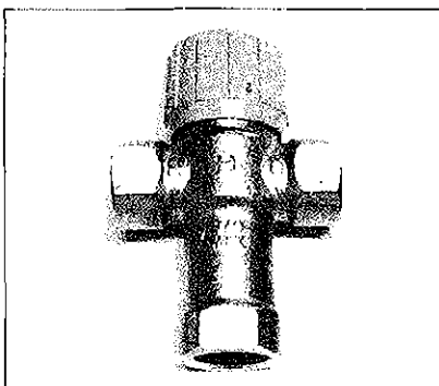
Adjust Thermostatic Mixing Valves at each point-of-use to 120°F or lower.
