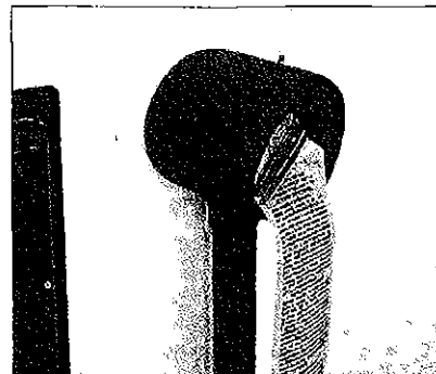
Make sure the insulation does not interfere with the T&P Relief Valve's operation.
